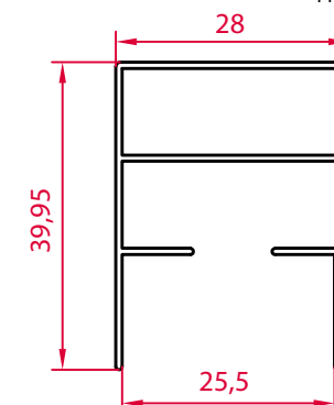
DE 1858 OKVIR VELIKI FRAME LARGE
