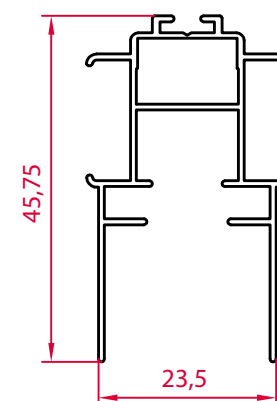
DE 1858 KRILO VELIKO SASH LARGE
