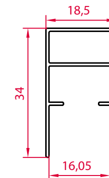
DE 1858 OKVIR MALI FRAME SMALL
